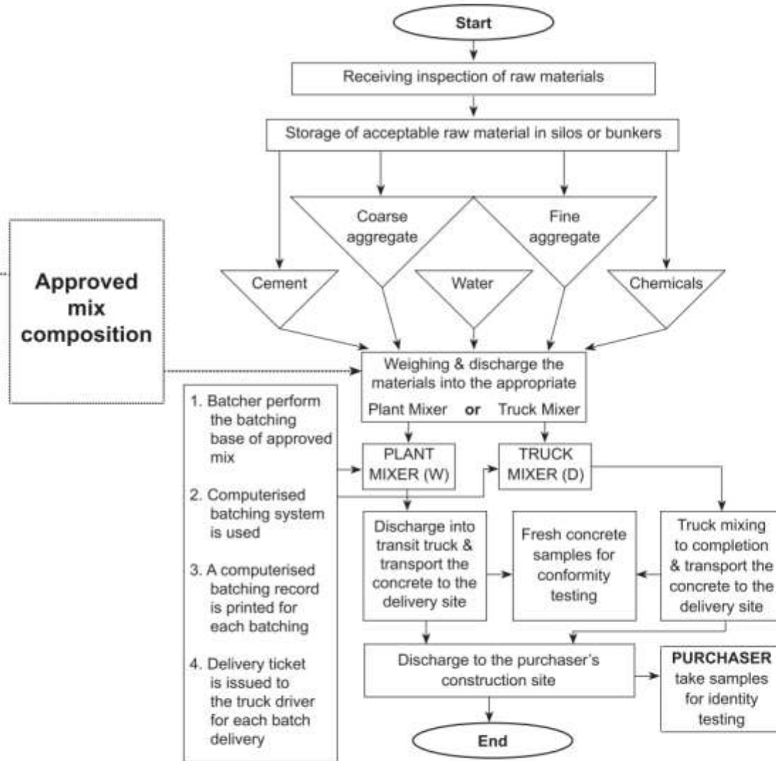
General Schematic Flowchart of RMC Manufacturing and Delivery Process
