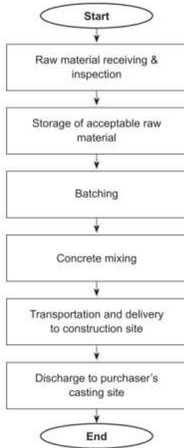
Simplified Flowchart for Manufacturing and Delivery Process
