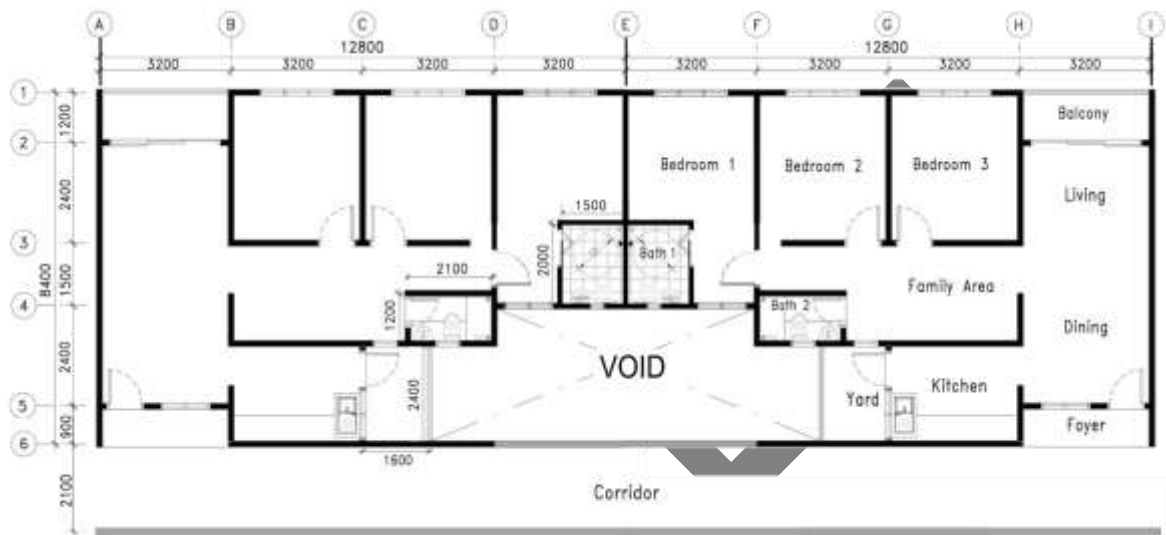
Floor Layout for Type 1
