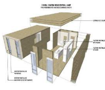
d) Prefabricated timber unit
