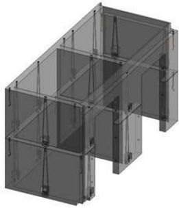
a) Prefabricated lift core module
