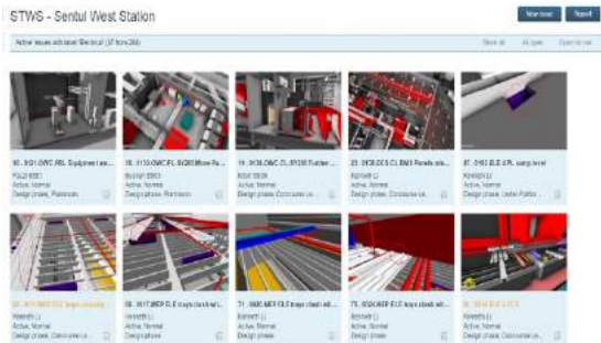
d) Screenshot of BIMCollab issues during the design stage
