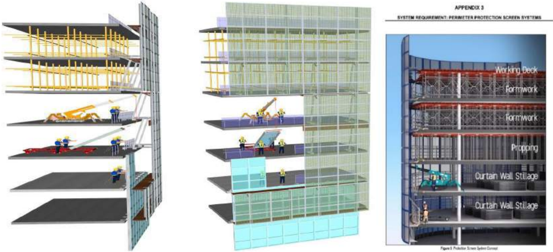
a) 6.5Floor Protection System x-climb 60
