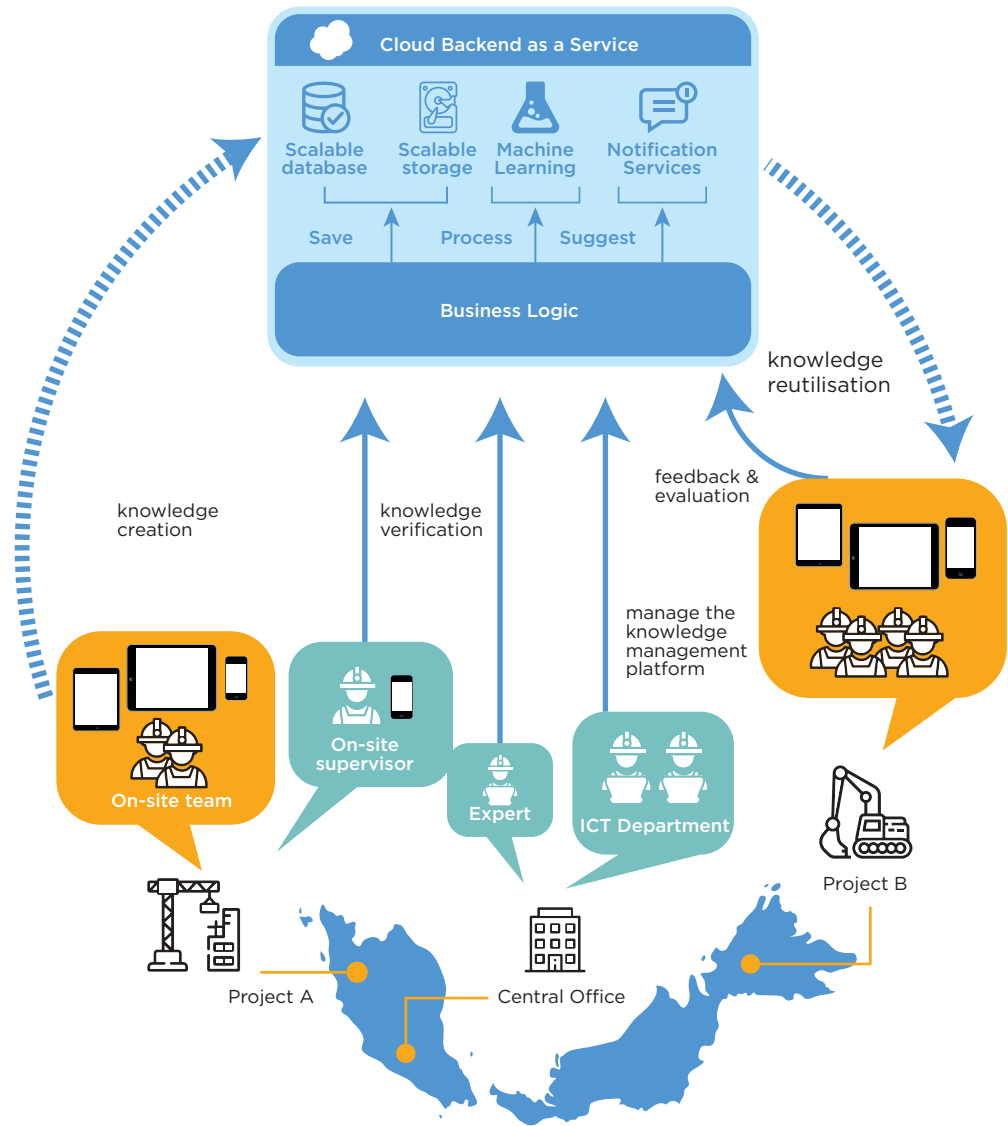
Figure 3.4 An example is a cloud and real-time collaboration workflow within an organisation.
