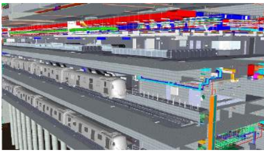
b) Sample station federated model
