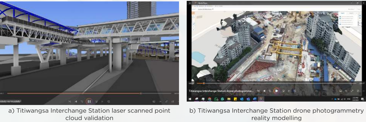
Figure 5.21 Laser Scanning and Photogrammetry Application Used for Construction Stage
