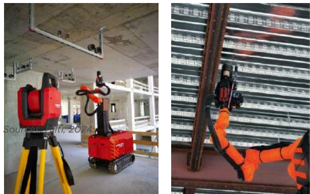
Figure 4.24 Hilti Jaibot used to mark and drill holes, relieving construction workers from the strenuous task of overhead drilling.
