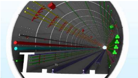
a) Sample tunnel federated model
