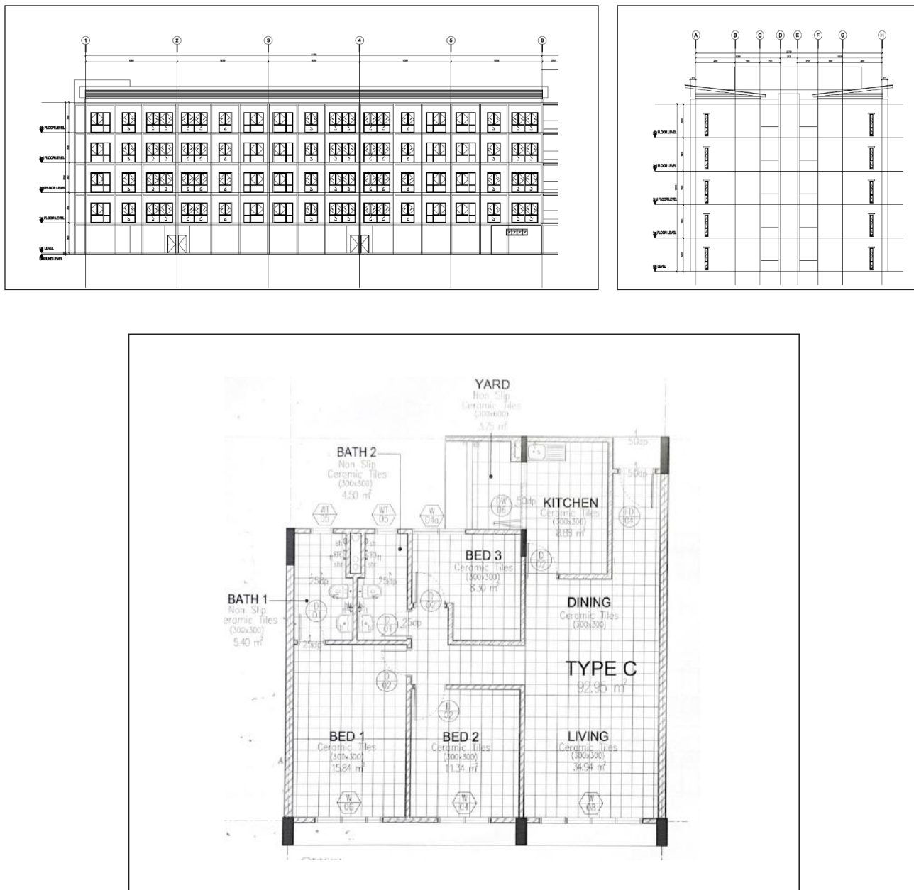
Figure 4.9. Typical layout for Pangsapuri Aurora
