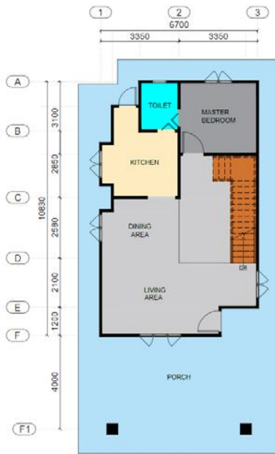
MyIOS Single House 2-storey P12 Ground Floor Plan Layout
