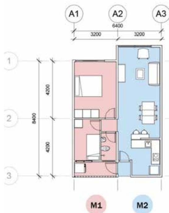
DeLIGHT Homes Apartment 2-Bedroom Flat Floor Plan Layout
