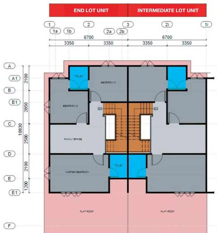
MyIOS Terrace House 2-storey P07 First Floor Plan Layout
