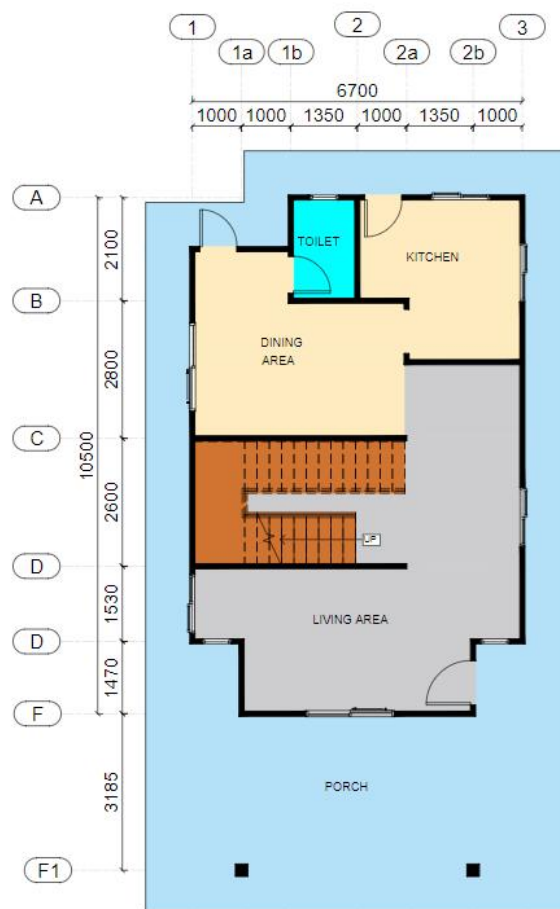
MyIOS Single House 2-storey P13 Ground Floor Plan Layout
