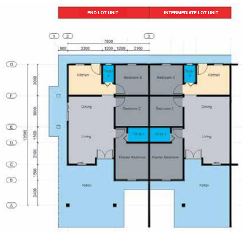
MyIOS Terrace House 1-storey P08 Floor Plan Layout
