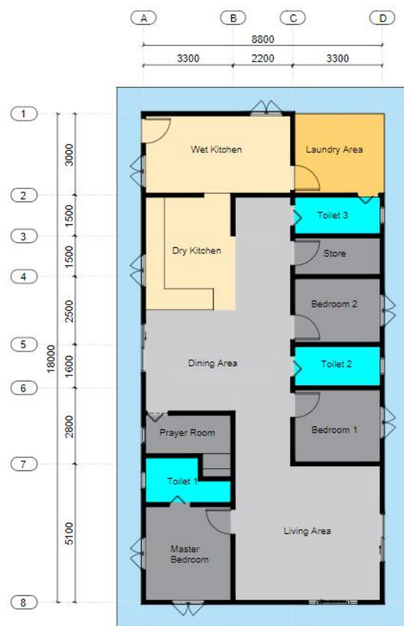
MyIOS Single House 1-storey P14 Floor Plan Layout
